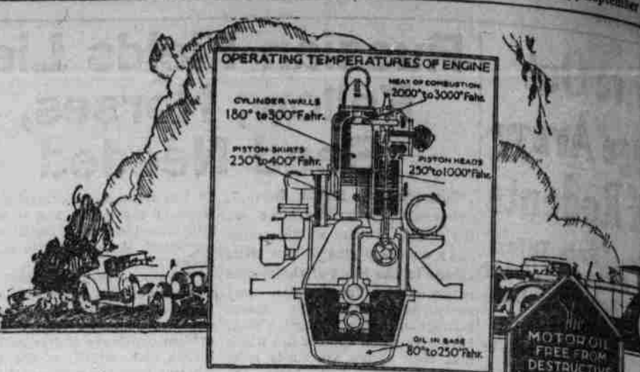
The combustion of gasoline generates a heat of about 3000 degrees Fahrenheit. Cylinder walls operate at about 300 degrees. Lubricating oils break down under this intense heat, impairing the piston oil seal.
