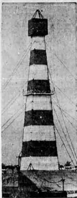
WHISPERING WELL — This striped structure stands on the outskirts of Maracaibo, Venezuela's second largest city. It's an oil-drilling rig fitted with a red and white "anti-sonic" shirt, which reduces roar of drilling operations to a mere whisper, so weary residents can get their sleep.
