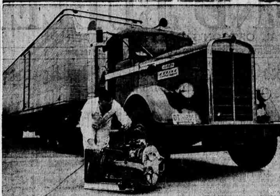
PINT-SIZE TURBINE FOR KING-SIZE TRUCK —A mechanic at the Boeing Airplane Co., Seattle, Wash., shows the 200-pound, 175-horsepower gasoline turbine engine which is being used successfully to power the ten-ton truck behind him. The new engine, not yet ready for installation in your auto, occupies only 13 per cent of the space required for a conventional 200-horsepower gasoline engine. It runs equally well on gasoline, kerosene, light or heavy fuel oil, and has been test-run on bottled gas. Boeing engineers say the gas-turbine engine soon will compete with piston engines both in autos and trucks.
