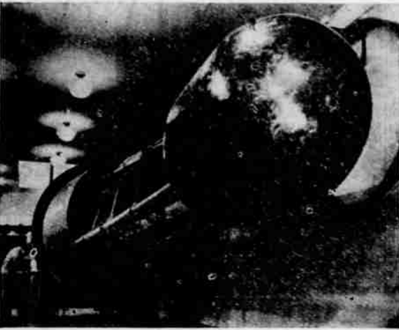
8,000,000-VOLT ATOM SMASHER—This huge atom-smasher, weighing 20 tons, will soon be in use at Notre Dame University in Indiana, where its 8,000,000 volts will serve for experiments.
