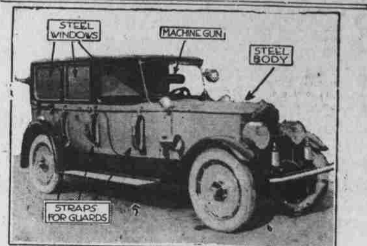
* Governor General Tsan Tso-Lin of Manchuria, values his life too highly to take any chance with bandits. This fortified Packard limousine has been shipped to him from New York. Its frame is of armor plate and it has heavy steel window shades. A machine gun is part of the equipment. The three belts attached to the side are for guards with rifles.
