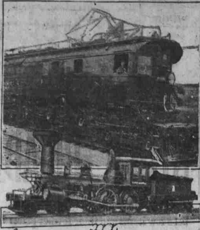
CHICAGO—The world's most powerful electric locomotive is on exhibition at the Chicago, Milwaukee & St. Paul Terminal here. It is 88 feet long, has 4200 horse-power, can pull a train 65 miles an hour and cost $112,000. It is the latest step from the first steam locomotive of 90 years ago. The contrast can be seen by the two photographs.
