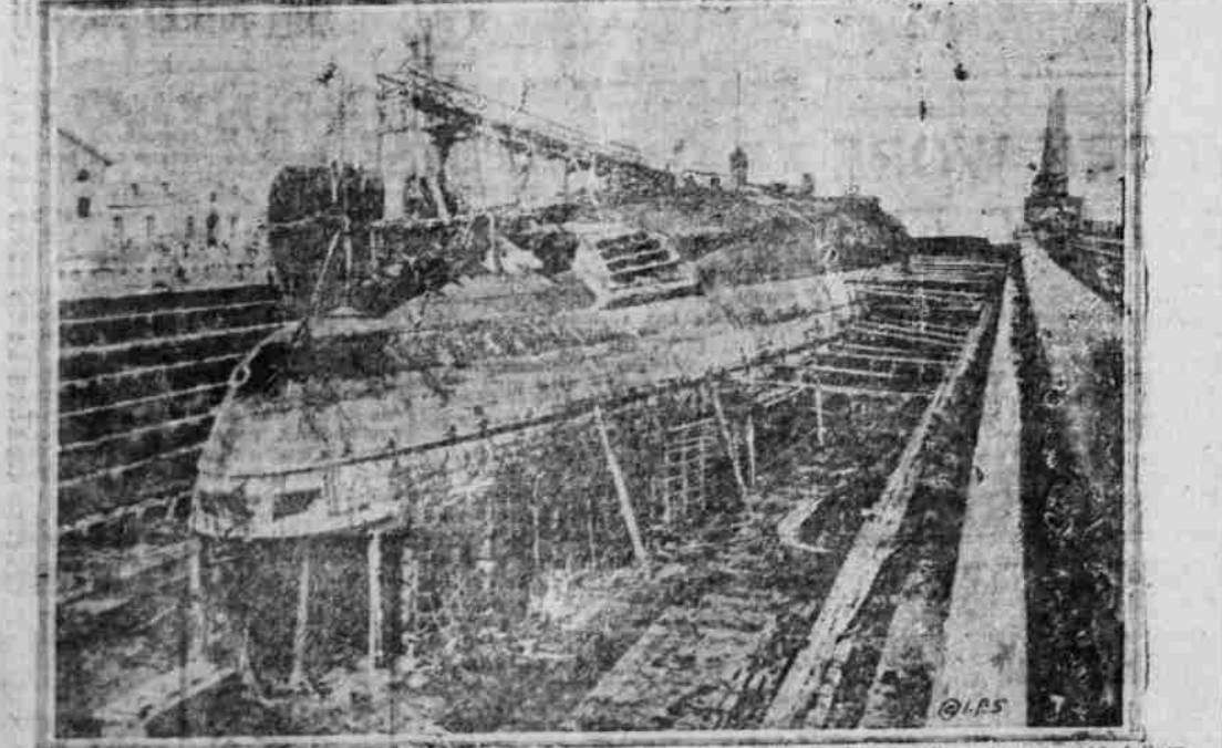
Italian engineers are confident that the dreadnaught Leonardo da Vinci, which sank on Aug. 2, 1916, following an internal explosion of the munition stores, will be perfectly serviceable when she has been re-launched from drydock at Taranto. The battleship turned turtle when she was raised upside down and taken in that position to Taranto. This photograph shows her still upside down, in drydock. Naval engineers say she will right herself when she goes into the water. The port side of the Leonardo da Vinci is seen here as she rests on timber supports, the stern being in the foreground.
