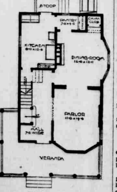
FIRST FLOOR PLAN. showing four and a half inches to the weather, making a lap over of one and a half inches. The first floor contains a large recep-
