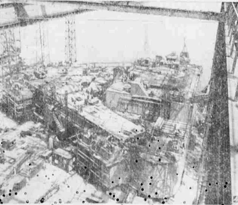
SEA RADAR TOWER NEARS COMPLETION —The first of the offshore radar, plane-detecting towers is nearing completion at the Ford River shipyard at Quincy, Mass., and will be launched soon. The huge, glauco-brown steel platform, weighing 2,000 tons will be towed to sea and placed in position on a barge in the ocean on Georges Bank, about 110 miles east of Cape Cod. The towers will take the form of a gear chain, strung along the Atlantic coast from Norfolk, Va., to New Brunswick, distance of 1,000 miles.
