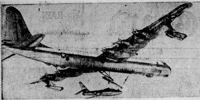
'MOTHER SHIP UNIT'—The United States Air Force has revealed plans for the first operational "mother ship" unit, teaming F84 jet reconnaissance fighters from the Great Falls, Mont., Air Force Base with giant B36 bombers from the Spokane, Wash., Fairchild Air Force Base. Speedy fighters are carried inside bomber, can be launched and recovered in flight. Jet makes connection from apparatus on belly of bomber. B36, world's largest bomber, has a range of some 10,000 miles.
