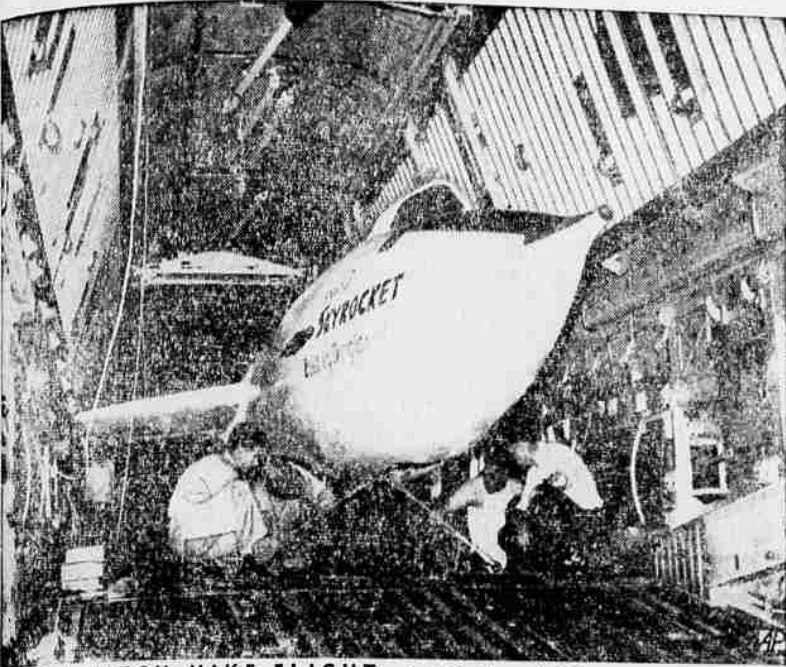
GET FOR HITCH-HIKE FLIGHT —A partly-dismantled Navy Skyrocket plane is hoisted down inside an Air Force Globemaster at El Segundo, Cal., for a flight to Washington.
