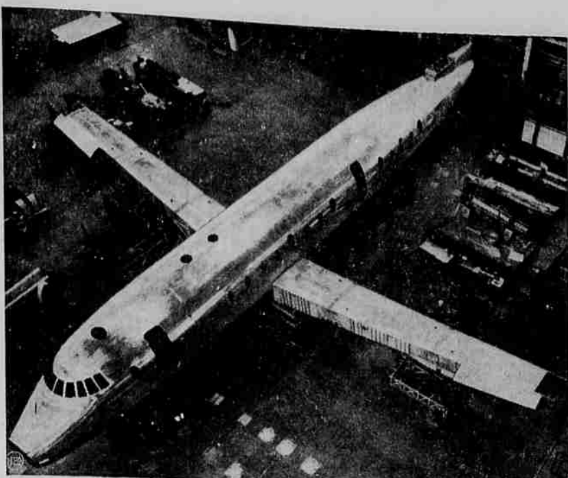
NEW WINGS FOR BRITAIN—The huge, new Britannia airliner takes shape at the Bristol Airplane Company's plant in Filton, England. First of 25 of the 107-passenger ships on order for British Airways, it will have a wingspan of 140 feet, will be 114 feet long, and 38 feet 8 inches high. Designed to cruise at 370-miles-per-hour the big ship will cost $1,540,000.
