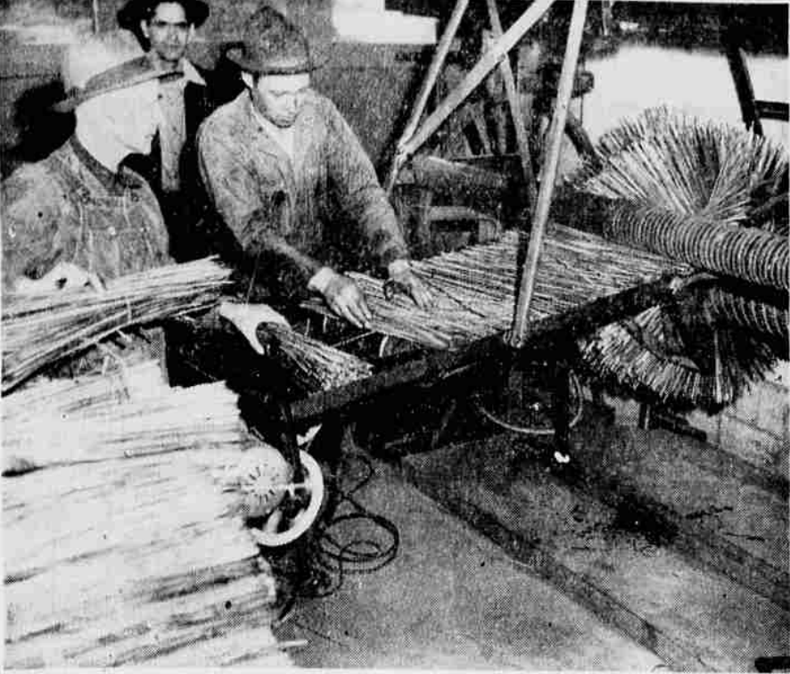
IT LOOKS SIMPLE, and it actually is, but this is the only automatic street-broom rebuilding machine in the nation. It was invented by Eugene's street superintendent W. J. Mullins (center background), and built at the city shops with the help of Claude Jackson (left) and Bill Seavy. Now the three have applied for patents and have a Seattle equipment firm making duplicates for sale to other cities. Streets brooms wear out after sweeping about 250 miles along the curbs. Hand rebuilding here used to take 12 hours of strenuous effort. The machine, however, does the job in about eight minutes.
