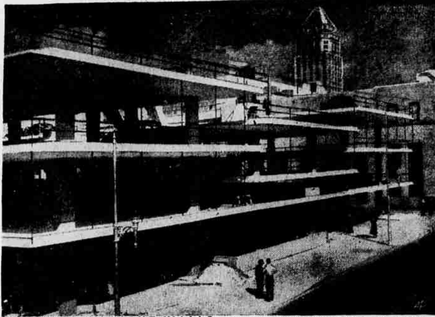
BUILDING WITHOUT WALLS — Made of poured reinforced concrete, without walls, and three "decks" high, this parking garage in Miami, Fla., has a capacity of 360 automobiles.
