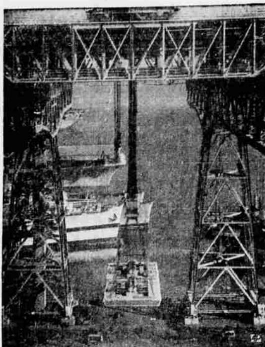
BIG CRANE AT WORK — A concrete, steel and lead slab, weighing approximately 630 tons, is lifted off the ground at the Hunter's Point Naval Shipyard at San Francisco by the world's newest and most powerful crane.
