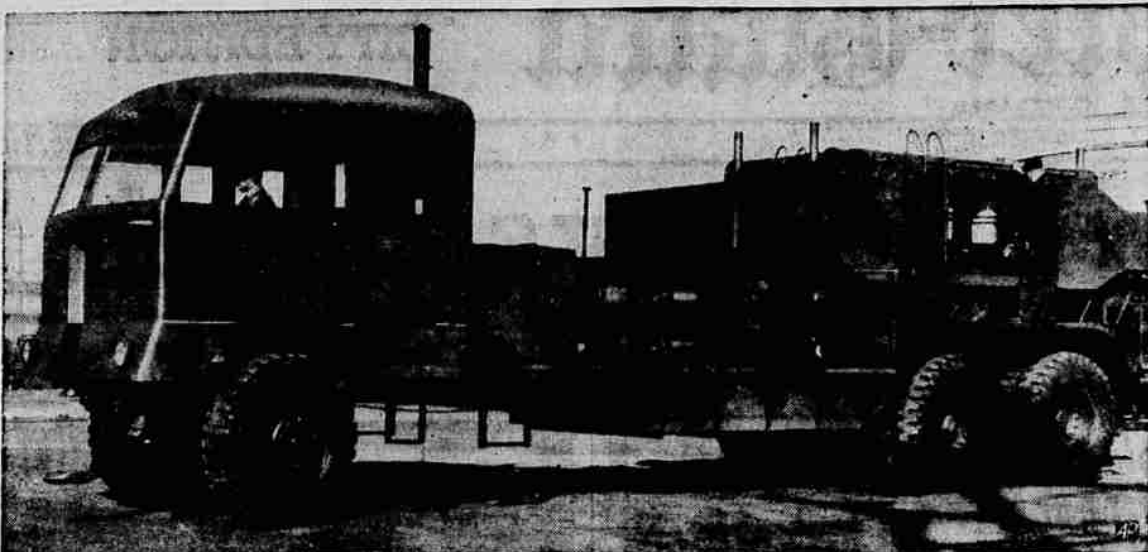
ARMY DYNAMOMETER-TRUCK —This 60-ton, 40-foot monster was designed to measure the tractive strength of the Army's latest tanks over the ordnance department's rugged proving grounds at Aberdeen, Md. It is electrically propelled.
