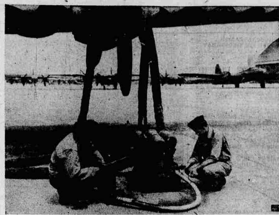
HEATER FOR HEATER —For weather which freezes the regular plane engine heater (right), Air Technical Service-Command designed small heater (left) to heat the big one.
