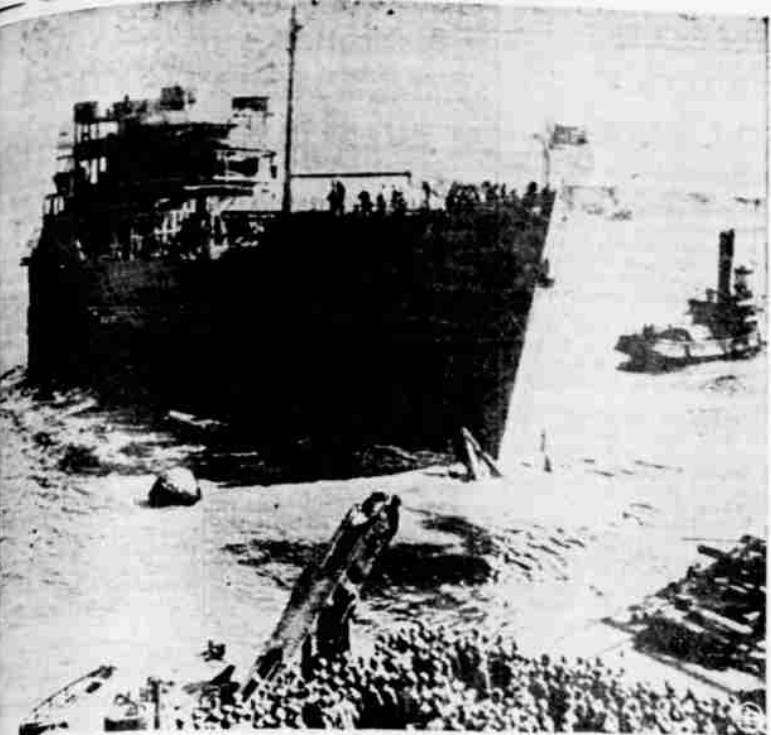
ENGLISH LAUNCH "HALF A SHIP" TO MAKE A WHOLE NEW ONE—Novel technique was this of half a ship at an English port. The forepart of a 12,000-ton tanker after striking a mine. Afterpart was towed to port where this new forepart was built and launched for a drydock "fitting."
