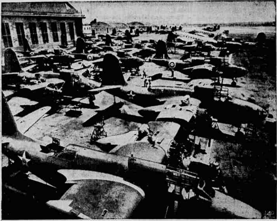
ATTACK BOMBERS ASSEMBLED OUTDOORS —More than 30 attack bombers, A-20-A's for the U. S. Army Air Corps and Havocs for Britain's Royal Air Force, undergo final assembly outdoors after coming off the production line at the Douglas Aircraft company plant at Santa Monica, Calif. This type of plane has been used as a night fighter by the R. A. F.
