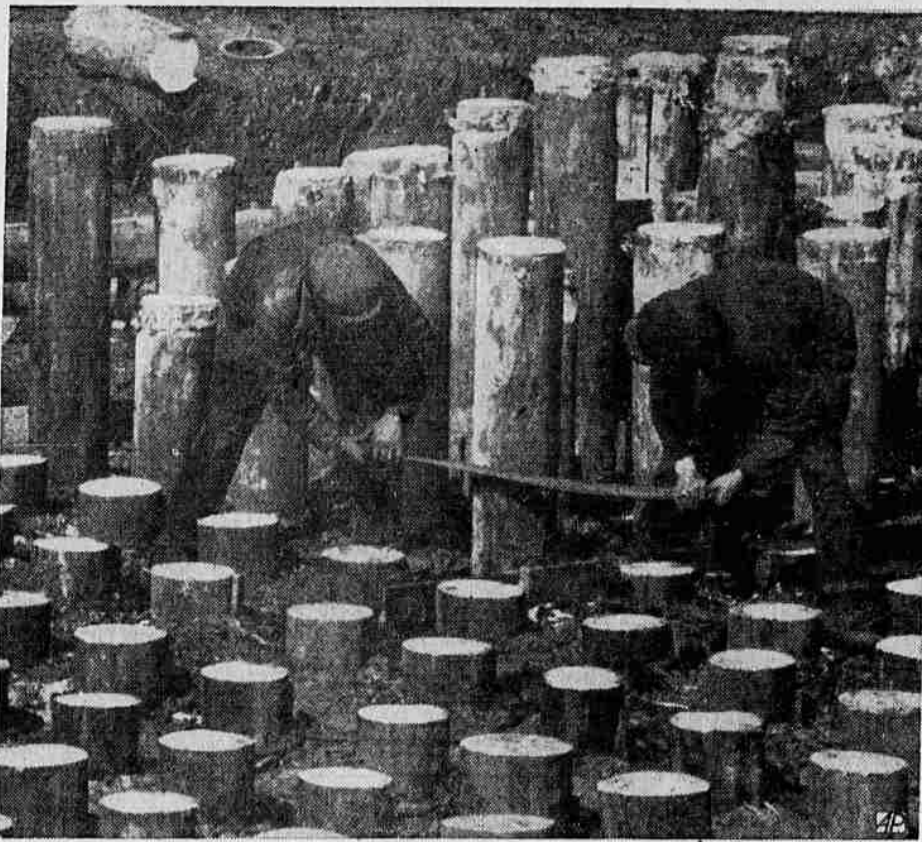
"ONCE over lightly!" Though this may look like a man's beard feels, view shows Holland road-building wherein deep-driven piles support road base. (A.P.-Universal Newsreel Photo.)
