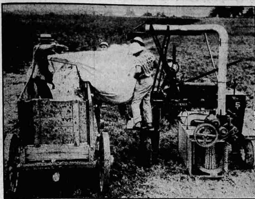
EFFICIENCY of the Rust cotton-picking machine, which may revolutionize agricultural methods in the south, was shown at the first public demonstration, given at the Delta experimental station at Stoneville, Miss. Here the machine is shown as it unloaded its harvest into a wagon, after a run through the field, covering a 1000-foot row in less than four minutes. The cotton, blown from the conveying pipe into the huge bag, came out whole and clean, and observers were highly impressed with the test.
