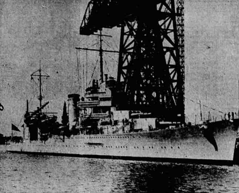
One of the newest of the U. S. navy's 10,000-ton "treaty cruisers," the U. S. S. Minneapolis, is pictured tied up to her pier following commissioning ceremonies in Philadelphia. Built at a cost of $11,000,000, the cruiser has a speed of 32.5 knots and will carry four airplanes.
