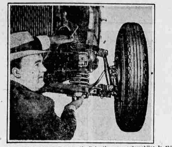
An example of the "knee action" in the new automobiles is this coil spring and lever combination shown on a front wheel of the new Plymouth, on sale at Brown Motor Company, Lane Auto, and Reid and Sawyer in Eugene. There is no front axle; the forward wheels act independently of each other and smoother riding results.
