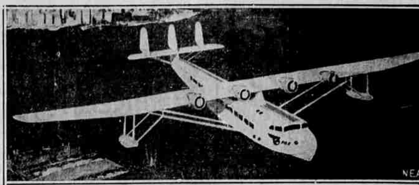
Col. Charles A. Lindbergh designed this new air transport marvel which the Pan-American airways will install in its regular Central and South American air service. It will carry 50 passengers, mail and freight, and is capable of scheduled transport operation over the longest water haul between the two hemispheres. There are many revolutionary improvements in structure embodied in the new plane.
