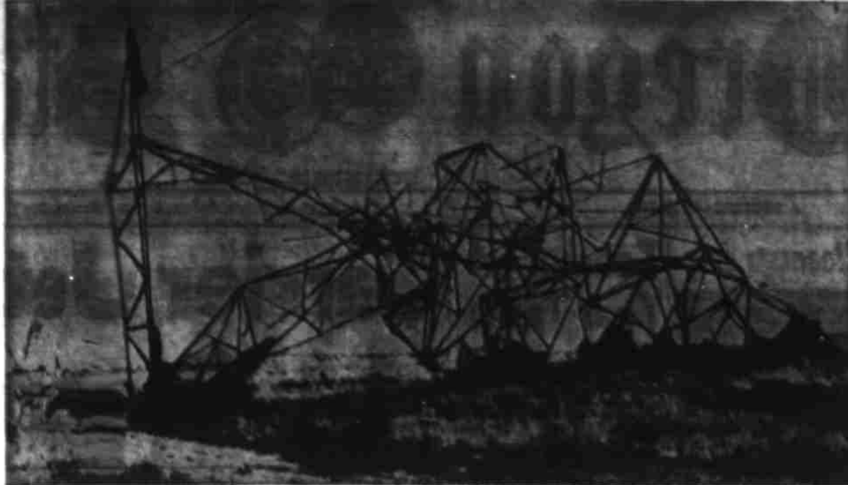
BOARDMAN, Ore., June 6—Winds of hurricane force struck Eastern Oregon areas in violent gusts Wednesday night, ripping to shreds a two-mile section of Boardman Power Administration lines. Shown in picture is one of 15 steel towers knocked over. Standing 60 feet high, towers weigh 60 tons and were built to withstand winds of 100 mph. (AP)
