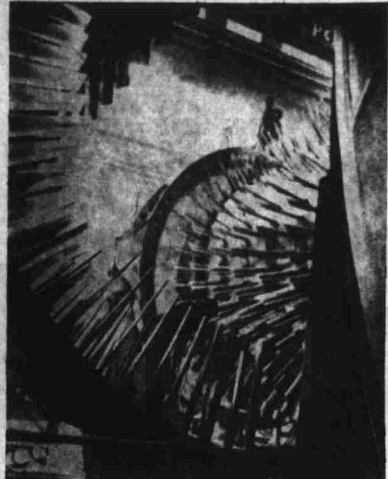
Lot of Wind CLEVELAND—Nation's largest supersonic wind tunnel was unveiled Tuesday by National Advisory Committee for Aeronautics. Tunnel can duplicate air speeds up to 3 1/2 times that of sound at altitudes up to 30 miles. Shown here are blades of main drive compressor which drives air through tunnel. (AP Wirephoto).
