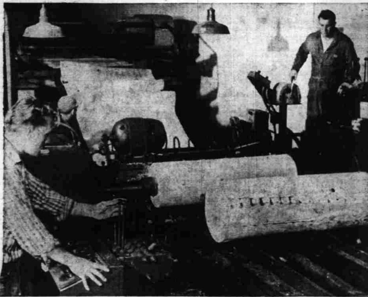
LYONS —There's little waste at the Lyons Plywood Division of the M and M Wood Working Co. Here the cores of peeler logs from the veneer lathe are cut in half and further "unrolled" on this smaller lathe, the veneer to be used as plywood crossbanding.
