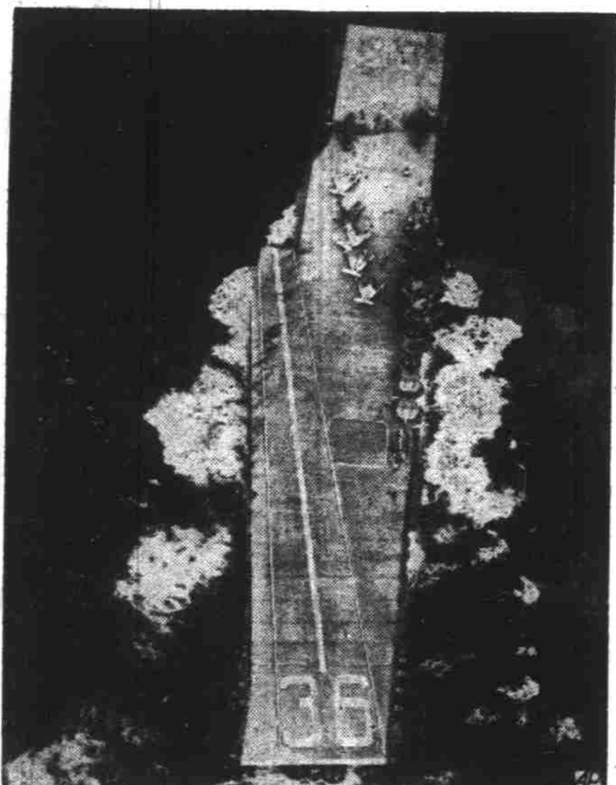
ANGLED FOR SPEED-UP — Angled deck of carrier USS Antietam, seen plowing through English Channel, is designed to permit landings and takeoffs on fore-aft axis or on angle.
