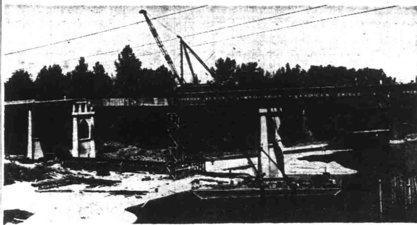
The final void in the span of the new Willamette River bridge in Salem was filled with steel Thursday. The girder on the north side is shown just as it was lifted into place, and the last girder for the south side is on the beach awaiting its trip upward. The bridge, which will carry west-bound traffic, is scheduled to be opened this fall.
