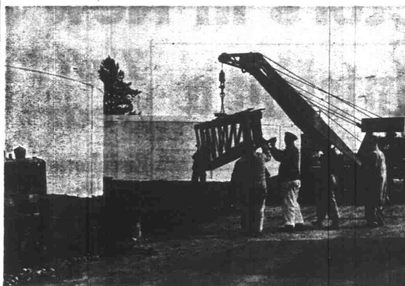
Steel girders to form the framework of covers for huge digesters at the new Salem sewage disposal plant on North River Road arrived this week after weeks of delay. The covers will be erected by the Chicago Bridge Co., and will weigh about 45 tons each. The two concrete digester tanks are 70 feet in diameter. The rest of the sewage treatment plant is complete. (Statesman photo.)
