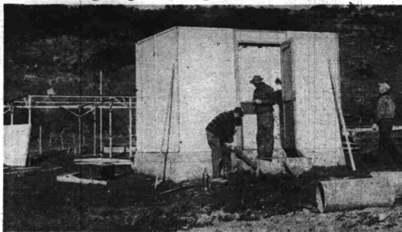
Final work in assembling the last of two prefabricated buildings to house radio equipment for Salem airport's new radio homing facility is shown above. Located just out of Turner about 4 1/2 miles east of the airport the radio marker will aid planes in landing during adverse weather conditions. At left is framework for a steel mesh anti-static system, and at right the radio building. (Statesman photo.)
