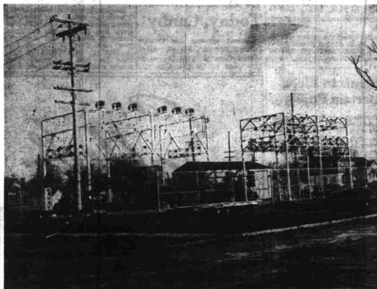
Gradual expansion of electrical service to northwestern Salem residents and industries will be provided by Portland General Electric Co. following completion of a new substation at Jefferson and North Liberty streets. Above is the steel framework in which will be placed two transformers with a total of 15,000 KVA capacity. Leading into the substation will be 57,000 volt lines, and outgoing will be 11,000 and 4,150 volt lines. Area to be eventually serviced will go east to Hollywood district, south to Market street and west to river; some also to the north. (Statesman photo.)
