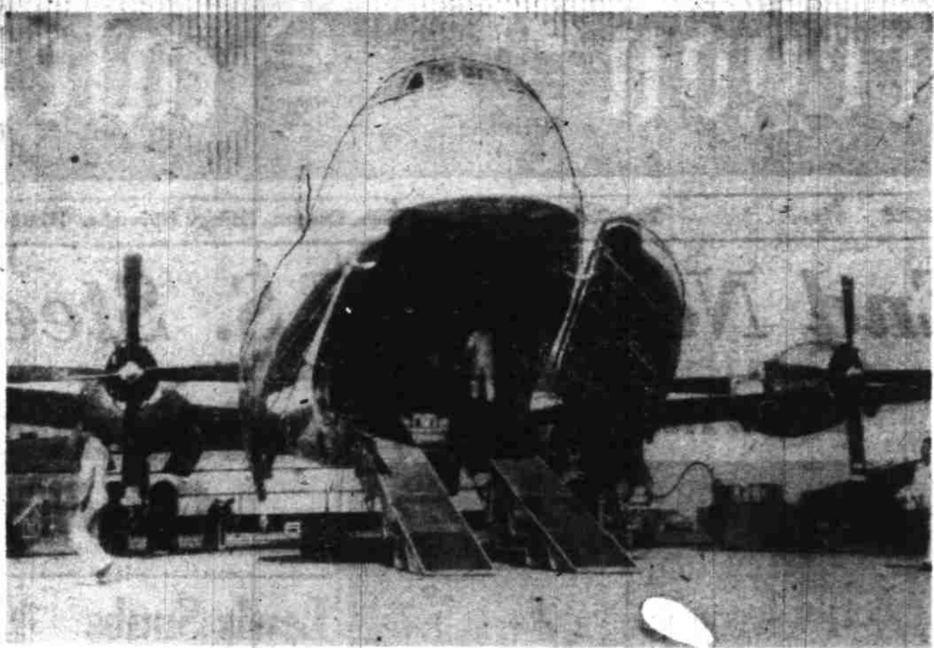
NEW YORK, Nov. 10—Tanks, field guns, bulldozers and fully loaded trucks can be driven up this loading ramp into the Air Force's new troop and cargo transport, the Douglas C-124 "Globemaster II." The clam-shell doors provide this loading hatch in the nose of the air force's largest production transport which was built at the Douglas plant at Long Beach, Calif. Loading of static cargo is facilitated by an electrically operated elevator which can be lowered from the center of the cargo section. (AP wirephoto from department of defense to The Statesman.)
