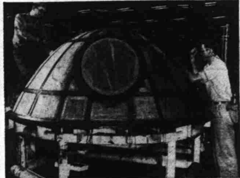
Bombardier's enclosure in last stages of glazing. Sealed during assembly, the enclosure is pressure tight after installation.
