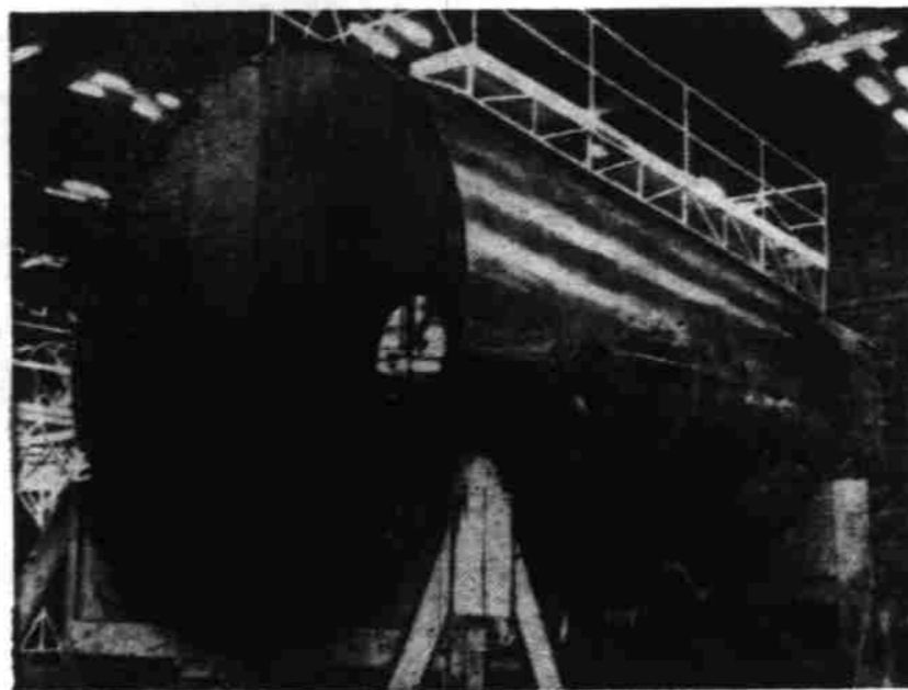
Tail structure aft of the bomb bay. It is now in a clean-up station. Next step will be its mating to the aft bomb bay.
