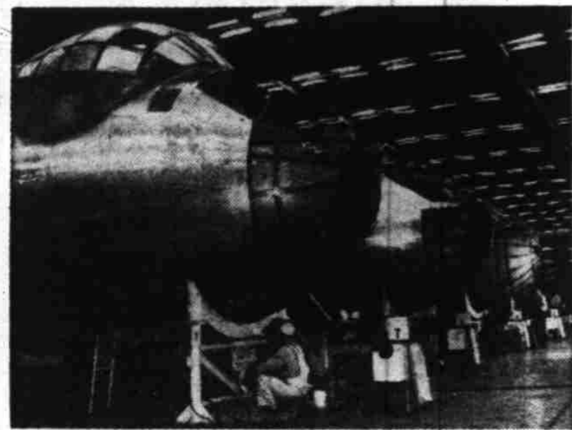
Clean-up nose-forward bomb bay primary line. Both the pilot's and bombardier's enclosures have already been installed.
