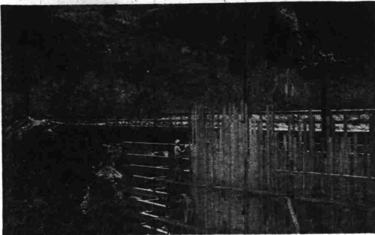
DETROIT, Sept. 12 (Special) -Workmen at the Detroit dam-site near here are shown constructing the upstream cofferdam which will soon divert the North Santiam river through a recently-completed diversion tunnel. A similar downstream dam will be built and a base for the main will be constructed in the dry river bed. The cofferdam above consists of a wooden crib filled with gravel and is to be completed in about two weeks. (U. S. Army engineers photo).
