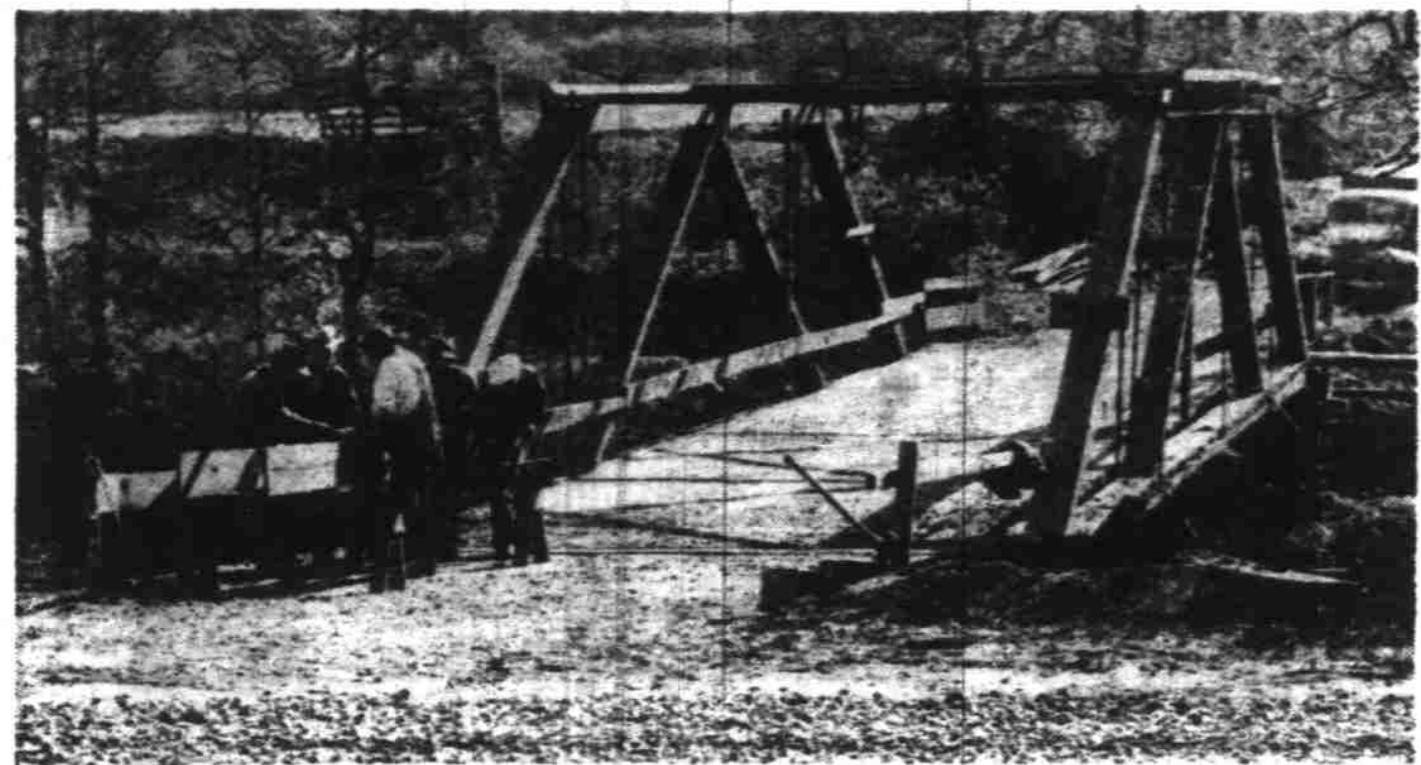
County road crews are at work constructing a new timber bridge to span Abiqua creek in place of the old Dunagan bridge above Silverton. The old covered bridge, 15 feet wide and 60 feet long, is being dismantled as shown above. The new span will be 20 feet wide and 65 feet long. Working in the photo above are Ted Kaenzel, foreman, W. L. Williamson, Arthur Tackmier, Menna Dalke and J. Robi, all of the Marion county bridge crew. (Statesman photo).
