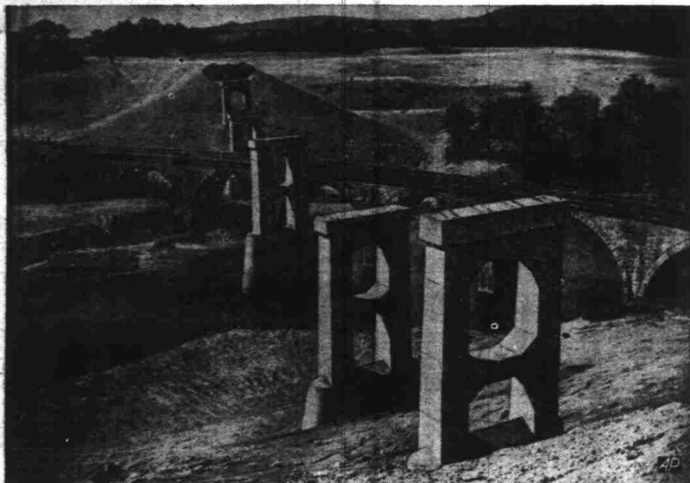
FLOOD CONTROL PROJECT —Army engineers built these piers over Bow River for railroad bridge to make way for $33,000,000 Conewago reservoir in western Pennsylvania. Old bridge runs beneath them. Conewago is seventh of 13 reservoirs designed to reduce flood dangers at Pittsburgh, 30 miles to west. System is part of Ohio river basin program extending into 12 states.
