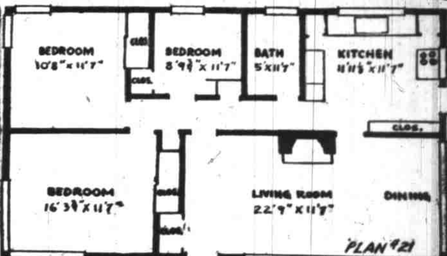
A contemporary styled bungalow combines simplicity of construction with smart appearance. This Plan No. 21 by the Modern Homes Council, Box 7761 Franklin Station, Washington, D.C., has been construction tested. The house shown above is built with ponderosa pine 10-inch tongue and groove siding. The plan covers 860 square feet.
