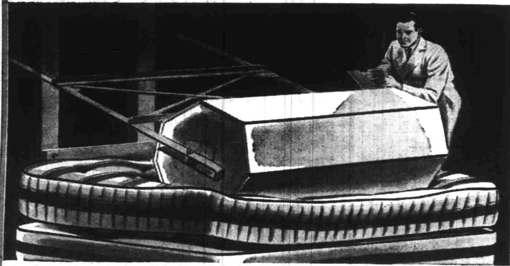
Mattress "Torture Test" at Laboratories of U. S. Testing Company
