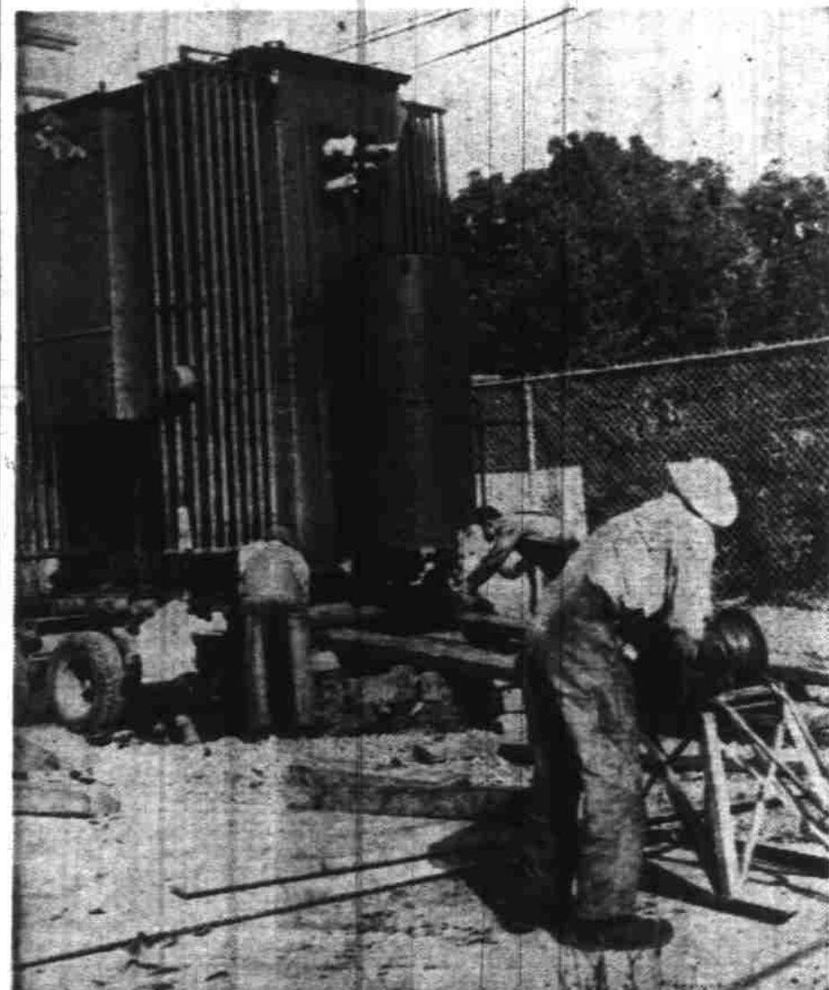
Installation of a new $34,000 General Electric transformer will be made at the University substation of Portland General Electric Co., located at Strand avenue and Mill street. Crews of the Wilhelm Hauling Co., of Portland, are shown above unloading one of the two transformers which arrived in Salem by rail after being on order more than two years. Each transformer will weigh 82,000 pounds when installed and filled with 2,635 gallons of special oil. The second transformer will be installed at a sub station to be erected at Fairmount and Miller streets in the near future. (Photo by Don Dill, Statesman staff photographer.)
