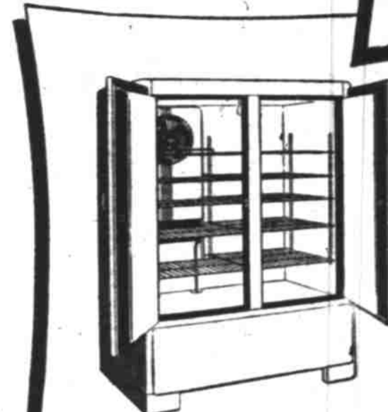
Model shown: F-30, forced air cooling. 30.7 cu. ft. cap.
