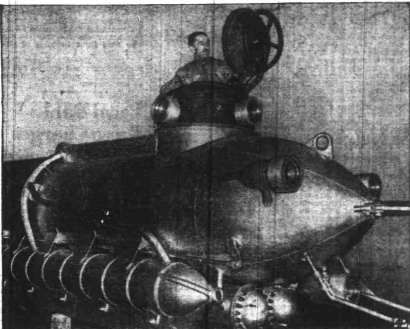
NEW ITALIAN SUBMARINE —Pietro Vassena stands in conning tower of midjet submarine he invented at his home at Lake Lecco, Italy. The craft, 25 feet long and 4 feet, 6 inches wide, was designed for scientific work and retrieving treasure from sunken vessels. Prof. Auguste Piccard, explorer of the stratosphere, will aid in testing the craft.
