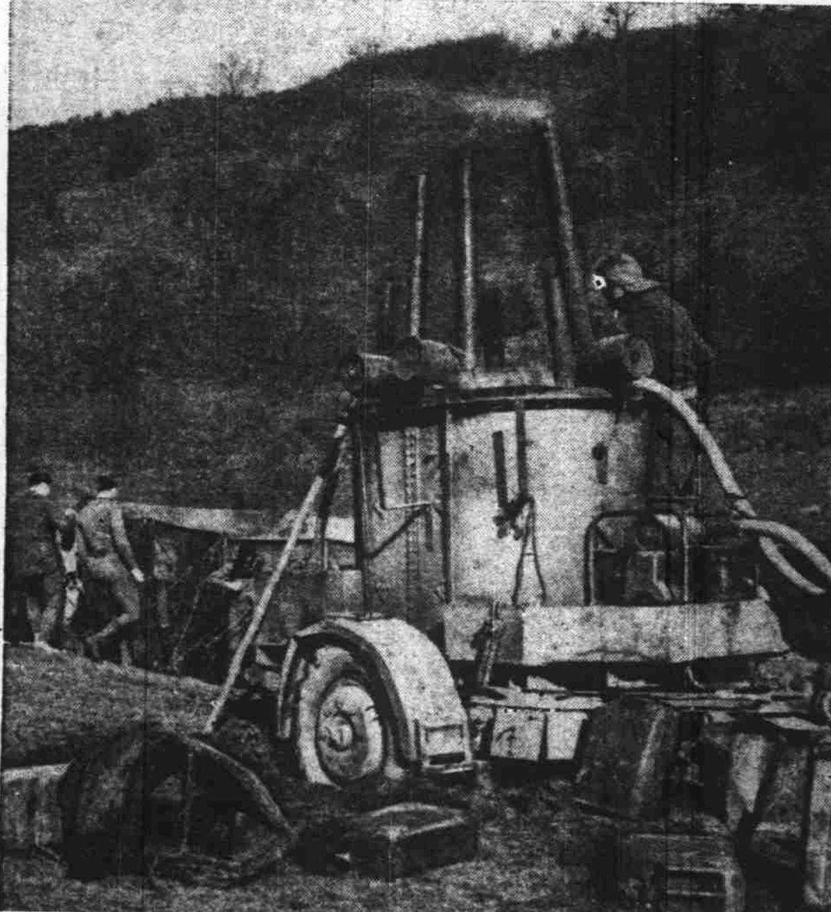
INGENIOUS PLUMBING—It looks a little like an anti-aircraft emplacement, but actually it's a field shower built of captured German materials by Tanks in Luxembourg.
