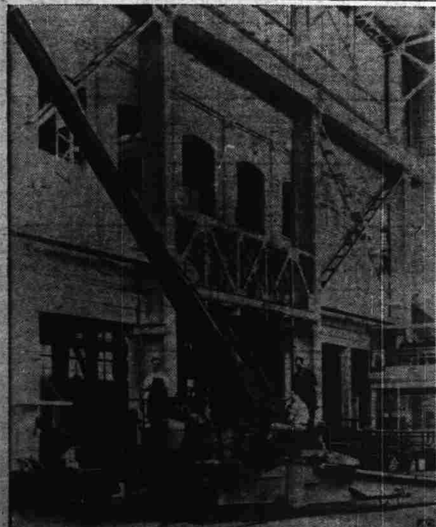
BIG GUN FROM YORK — Two York, Pa., companies collaborated to build this new 8-inch mobile gun for the U. S. Army, shown in final assembly in the S. Morgan Smith plant, normally making hydraulic turbines. The York Corporation, maker of refrigeration and air-conditioning equipment, was the partner. Assembly line ran through both plants.
