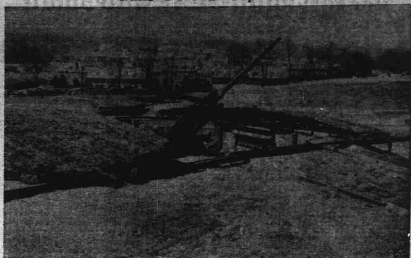
This 90mm anti-aircraft gun is in firing position as part of the wartime defenses of Washington. Imitation grass covers can be slid over the gun to camouflage it.—Associated Press Telegram.
