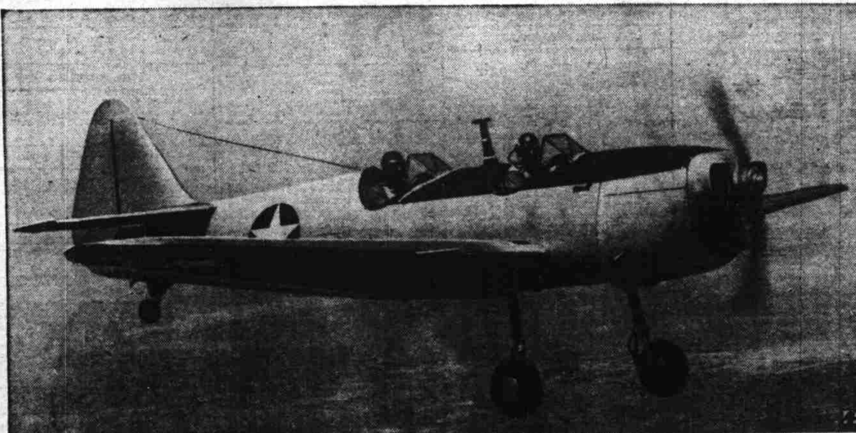
IT'S PLYWOOD. —This new Ryan FT-35 military primary training plane is made of plastic-bonded plywood. Aluminum alloys and all strategic materials have been eliminated except for engine cowling which is 2 per cent of plane's weight.
