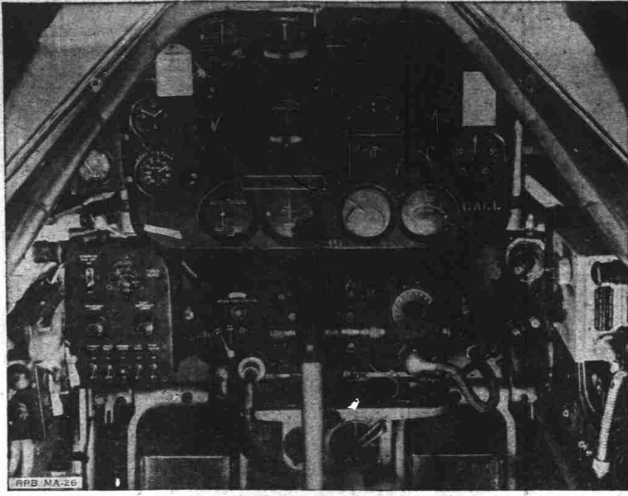
Above is shown the "installation" (or instruments) of a BT-9, the basic training airplane which US Army aviation cadets fly to win their wings. It's 79 gadgets, of which only 65 appear in the picture, range from a simple clock to a "selective gyroscopic drive control" and are a fine example of why Uncle Sam's pilots cannot "fly by the seat of their pants," as early pilots used to say. Instead, they must be highly educated and thoroughly trained so that they understand the functions of this maze of instruments, each of which is concerned with some highly technical phase of the science of flight.
