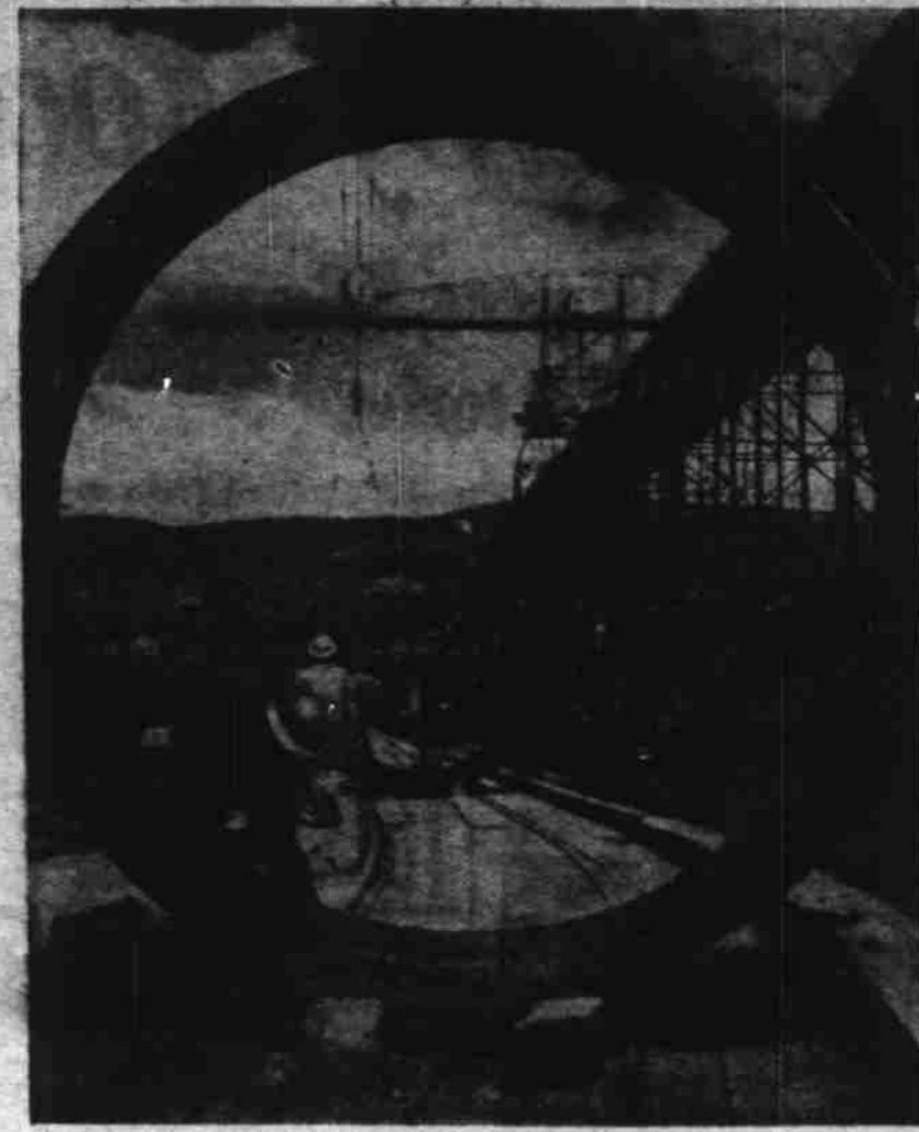
Two of the bell mouths for the permanent outlet pipes for the San Joaquin river at Friant dam are being inspected by workmen before being hoisted by cranes over the tall construction trestle and installed in the upstream face of the dam. The four outlets which will control the flow of the river will be 9 feet 2 inches in diameter and about 190 feet long. Similar outlets will regulate the flow into the Friant-Kern and Madera canals.
