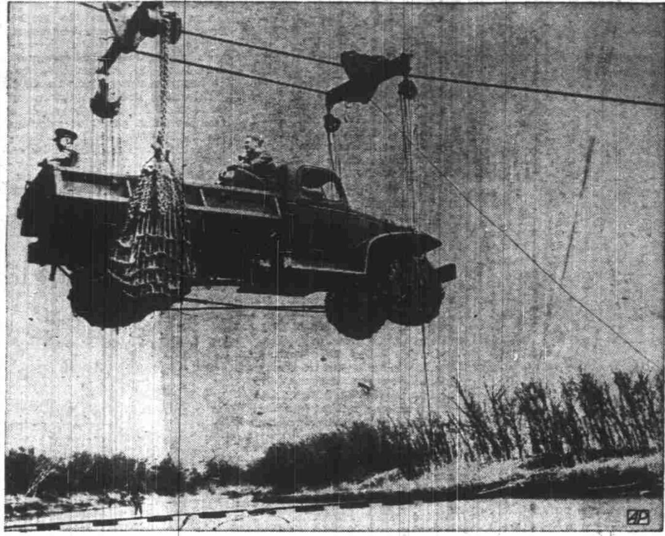
A new type cable bridge developed by Lieut. Col. R. B. Lord is given a successful trial at Fort Riley, Kan., as a seven-ton military truck is whisked up, over and across Smoky Hill river three hours after construction of the device was started. Below is a new type portable foot bridge with which the army is practicing.—AP Telemat.
