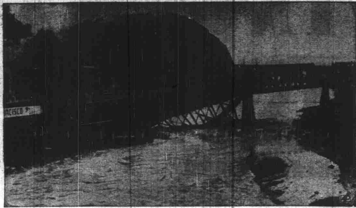
Swirling waters of the normally-dry Los Angeles river undermined an abutment supporting a Santa Fe railway bridge and caused a section 173 feet long to topple into the stream. Heavy rains sweeping southern California caused landslides which blocked highways and railway lines and brought the season's total rainfall to more than double the normal.
